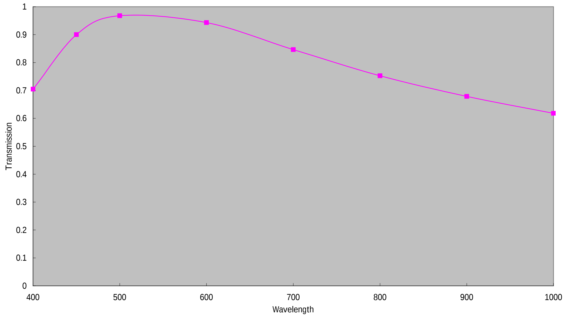
LM16JC (970) Transmission
