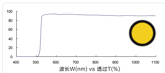
黄橙色长波通 520nm (Yellow-Orange longpass, FS03-LP520)
