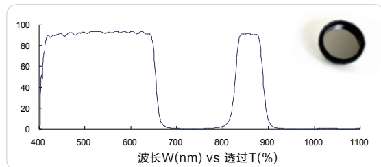
可见红外双带通 860nm (Dual bandpass, FS03-BPD86060)
