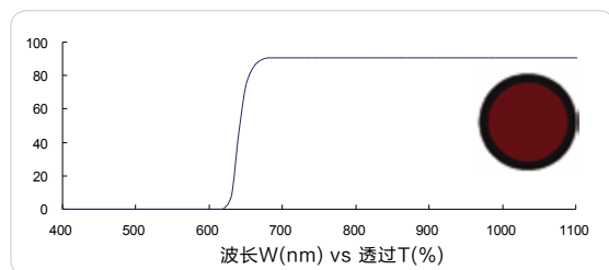
红色长波通 640nm (Red longpass, FS01-LP640)
