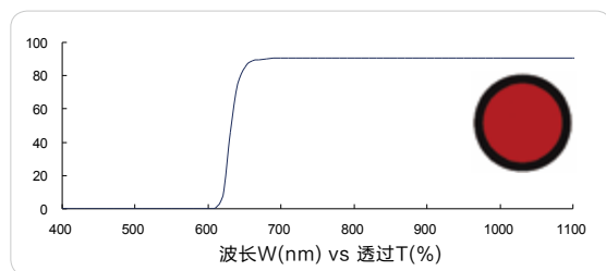
红色长波通 630nm (Red longpass, FS01-LP630)
