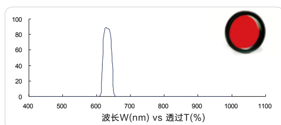
红色带通 630nm (Red bandpass, FS03-BP63030)
