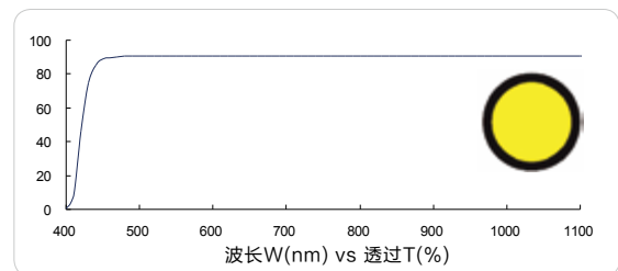
金色长波通 420nm (Violet longpass, FS01-LP420)
