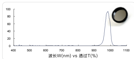
红外带通 980nm (IR bandpass, FS03-BP980)
