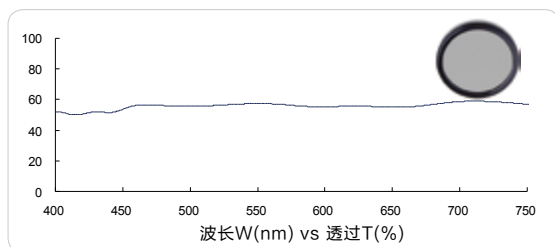
减光镜 (Neutral density (ND), FS03-ND2G)
