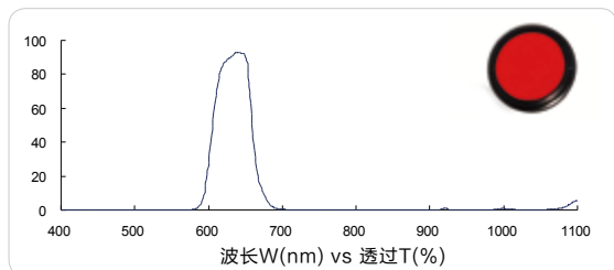
红色带通 635nm (Red bandpass, FS01-BP635)
