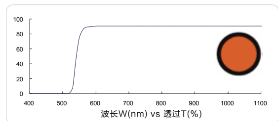
橙色长波通 535nm (Orange longpass, FS01-LP535)
