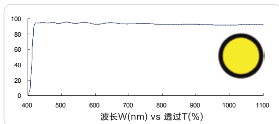
金色长波通 410nm (Violet longpass, FS03-LP410)
