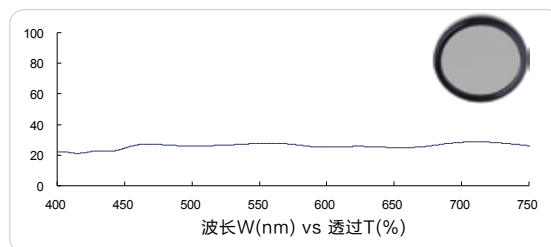
减光镜 (Neutral density (ND), FS03-ND4G)
