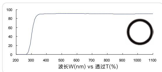
紫外长波通 330nm (UV longpass, FS03-LP330)
