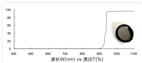
红外长波通 935nm (IR longpass, FS03-LP935)
