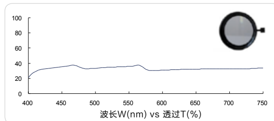
圆偏振镜 (Circular polarizer, FS03-PCR)
