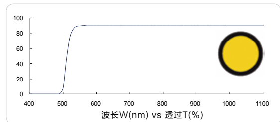
黄橙色长波通 510nm (Yellow-Orange longpass, FS01-LP510)
