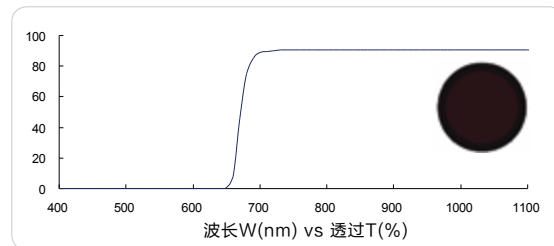
红色长波通 670nm (Red longpass, FS01-LP670)
