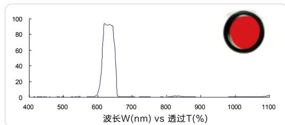
红色带通 635nm (Red bandpass, FS03-BP635)
