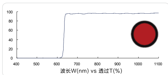
红色长波通 635nm (Red longpass, FS03-LP635)
