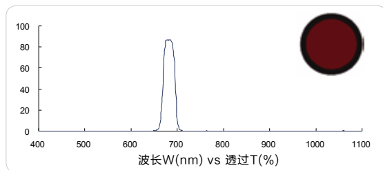
红色带通 680nm (Red bandpass, FS03-BP68030)
