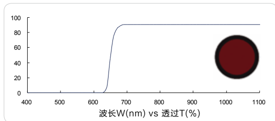
红色长波通 650nm (Red longpass, FS01-LP650)
