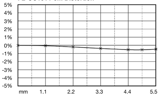
FL-CC1614-5M Distortion
